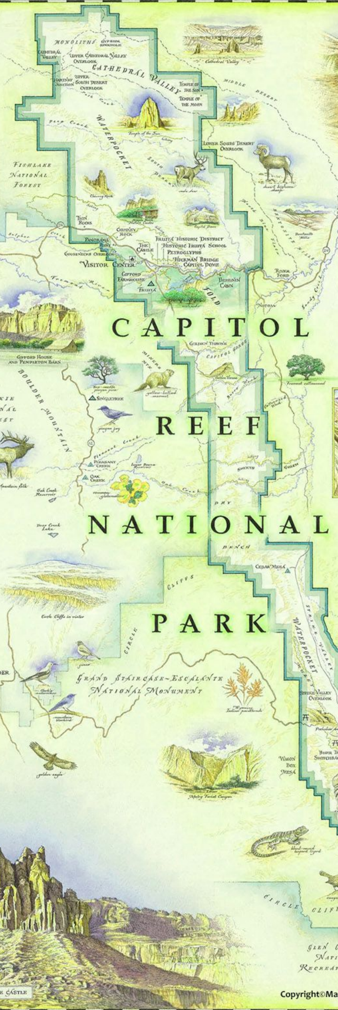
"WATERPOCKET FOLD" - A NEARLY 100 MILE LONG VALLEY IN THE EARTH'S CRUST, WAS FORMED BY PROCESSES OF DEPOSITION, UPLIFT AND EROSION.
